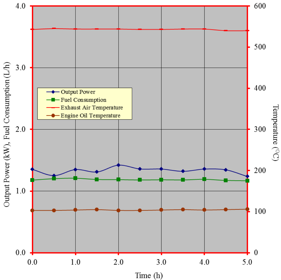
Figure 4. Performance characteristic curves during the continuous running test of the BRIGGS & STRATTON 122332 gasoline engine
