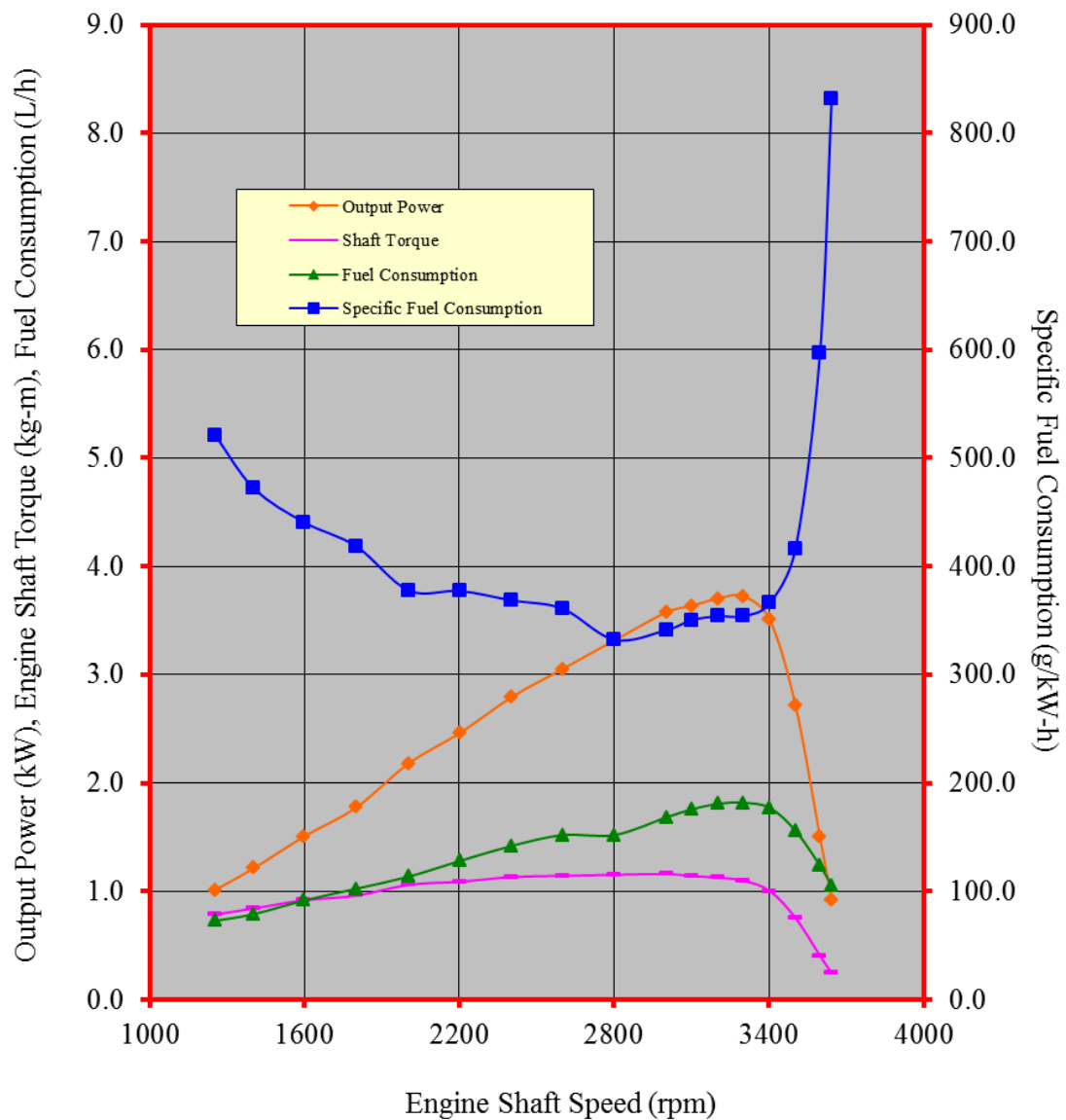
Figure 3. Performance characteristic curves of the BRIGGS & STRATTON 122332 gasoline engine
